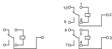
1C 2C Wiring diagram (Bottom view)
