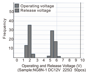
Operating and Release Voltage
