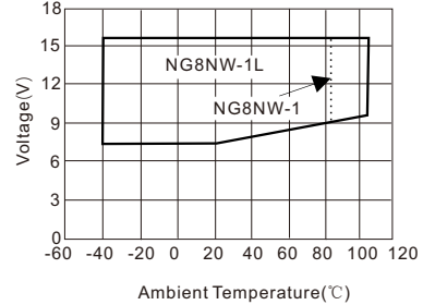
Ambient Temperature and Service Voltage Range(Cold Start)
