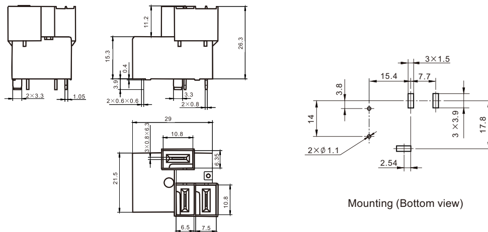
Dimensions(50A)
