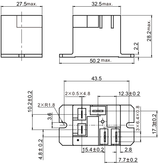
NT90TP 2 Mounting
