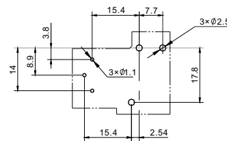
Double coils
