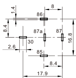
PCB type
