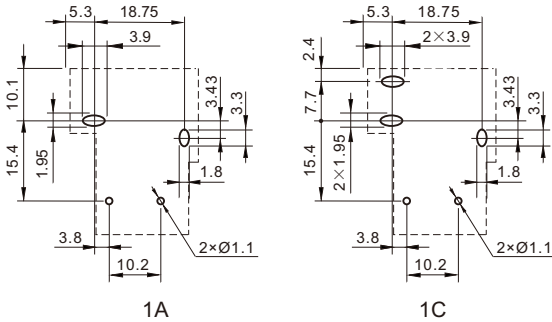
Mounting (Bottom view)
