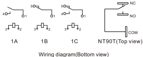
Wiring diagram(Bottom view)
