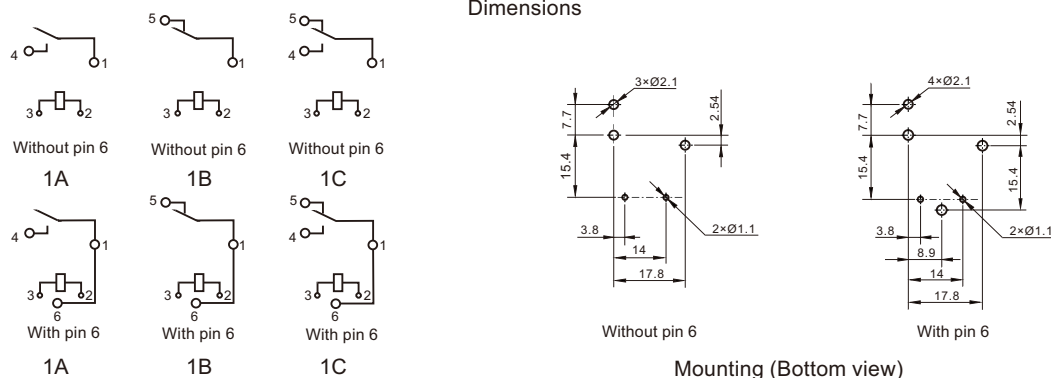
Wiring diagram(Bottom view)
