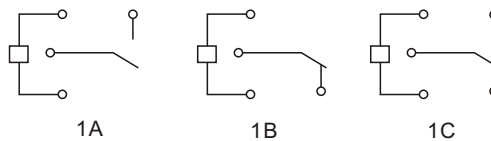
Wiring diagram(Bottom view)
